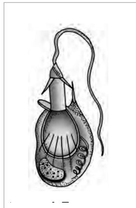
Fig. 4.7 - Diagrammatic view of Cnidoblast.
